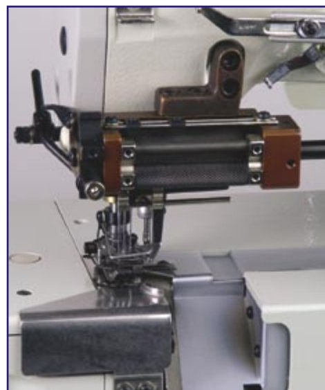
Top metering device on Global® FB 2553-64 TMD
