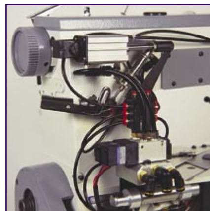
Pneumatic thread trimming and presser foot device
