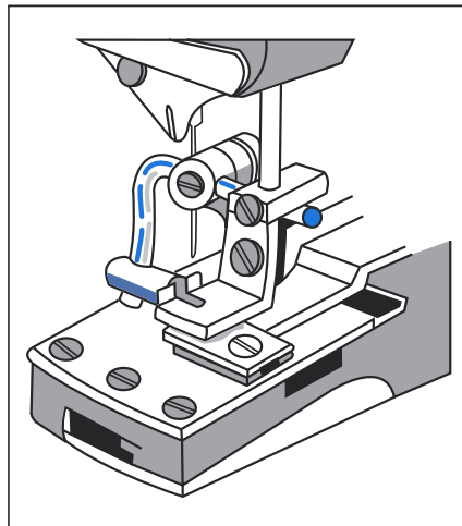
Attachment for shank buttons
