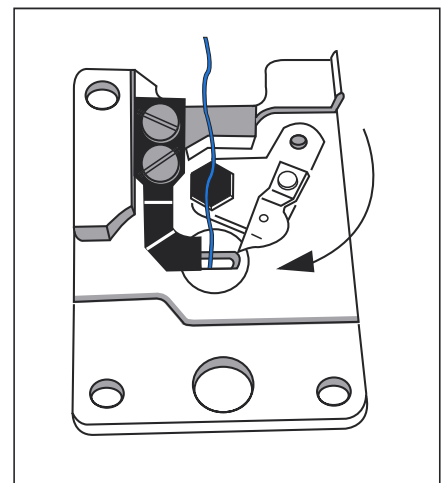
Thread cutter with a movable knife (BS 473)
